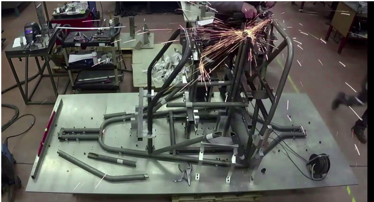
XC Cross Car welding
